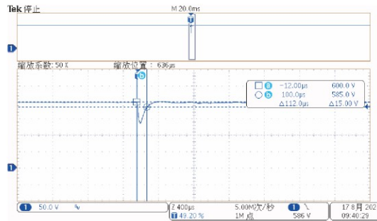
Transient full load, response time is 112\mu\text{s}
