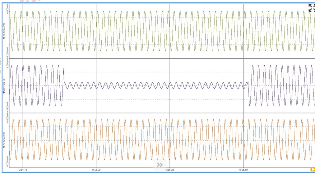
20% drop of phase B, time: 0.625s
