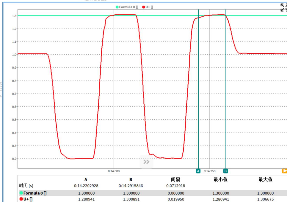
Voltage accuracy of two consecutive on-load high & low voltage ride through tests (longitudinal axis: 35kV per-unit value) \leq 2\%U_n
