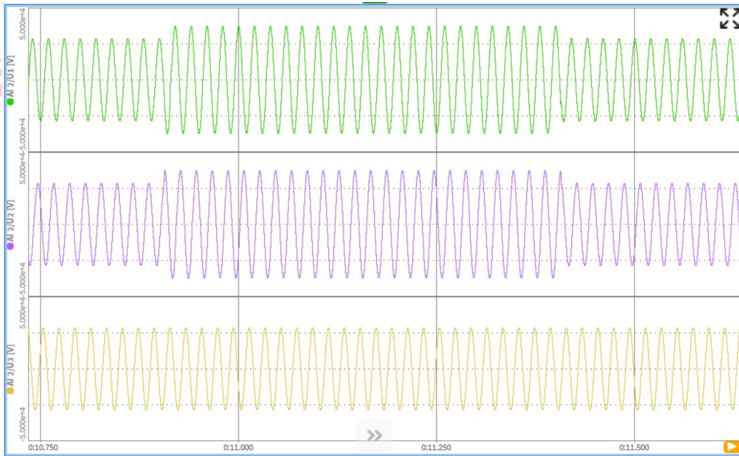
130% high voltage ride through test of phase A and phase B, time: 0.5s
