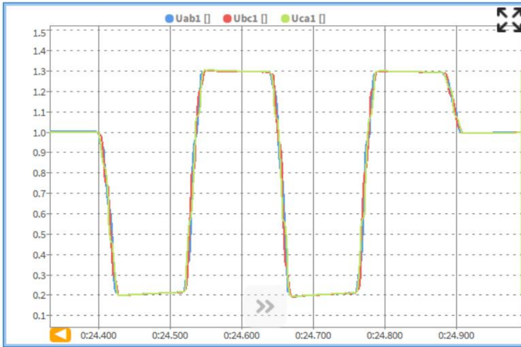
Two continuous no-load high & low voltage ride through tests (longitudinal axis: 35kV per-unit value)
