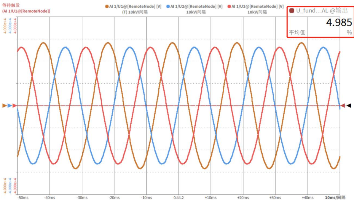
Three-phase unbalanced voltage waveform (degree of unbalance in the upper right red box)
