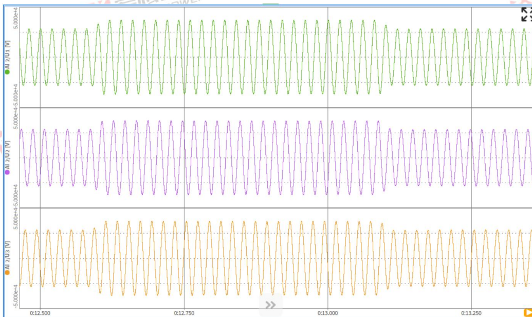
130% high voltage ride through test of three phases, time: 0.5s
