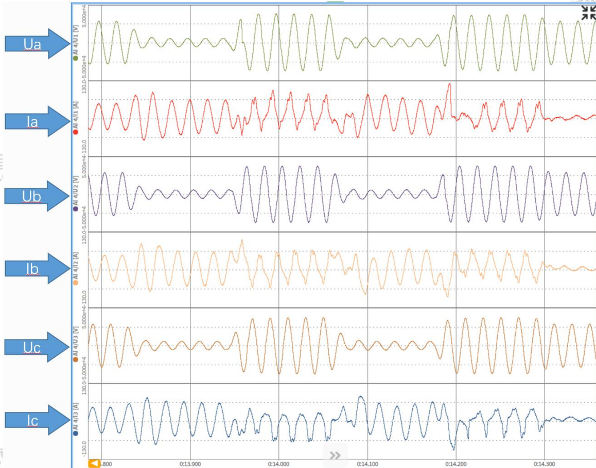
Two continuous on-load high & low voltage ride through tests
