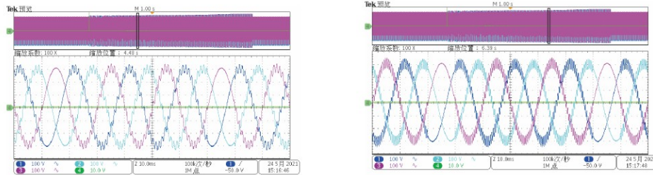
Inter-harmonic sweep
