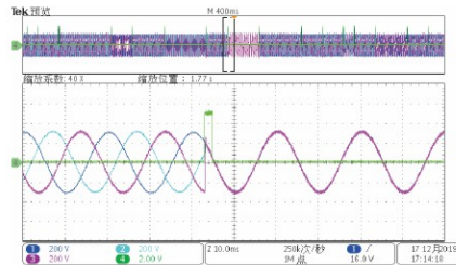
Phase Disturbance
