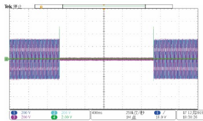
Voltage interruption
