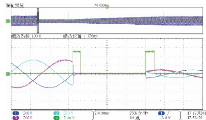
Three-Phase Low Voltage Ride Through
