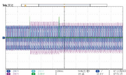
Single-Phase High Voltage Ride Through
