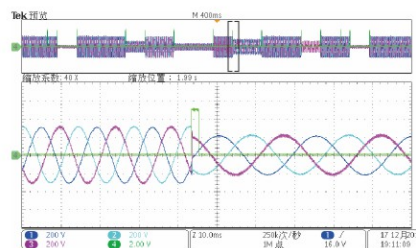
Frequency-voltage Variation
