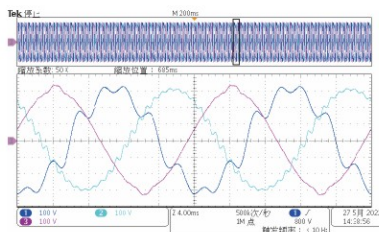
Harmonic Synthesis Waveform
