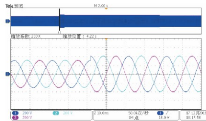
90° High Voltage Ride Through
