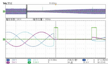
60° Low Voltage Ride Through
