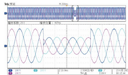
B-C Phase Switch LVRT
