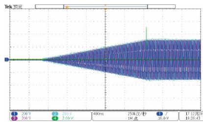
Slow recovery waveform
