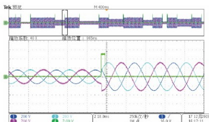
Voltage Disturbance
