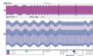
Inter-harmonic Synthesis Waveform
