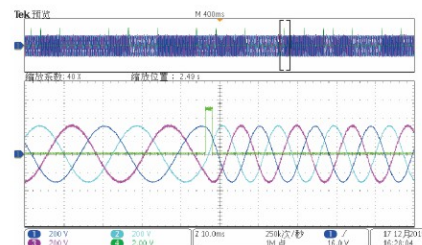
Frequency Disturbance
